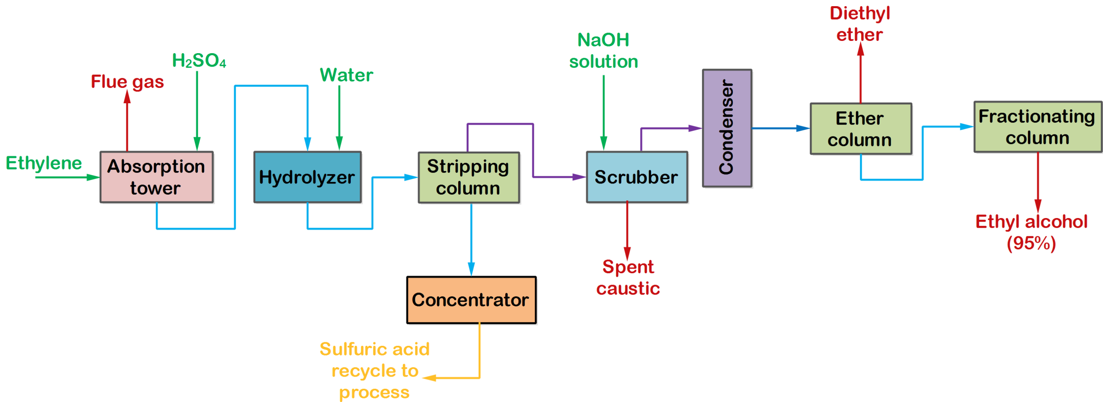
Figure: Manufacture of Industrial alcohol by esterification and hydrolysis
